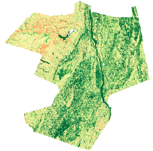
Random Forest
