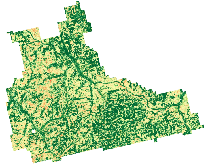
Random Forest
