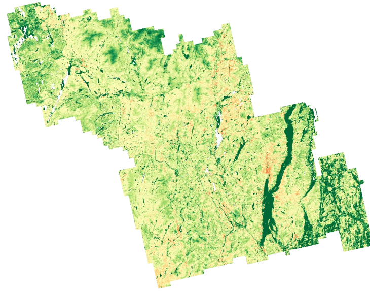
Random Forest
